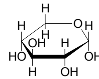
\alpha -D-Xylopyranose
