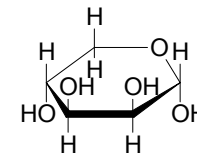
\alpha -D-Lyxopyranose
