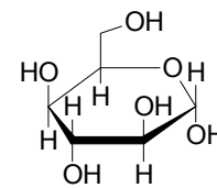
\alpha -D-Idopyranose
