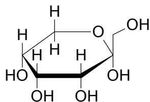
\alpha -D-Psicopyranose
