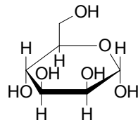
\alpha -D-Mannopyranose
