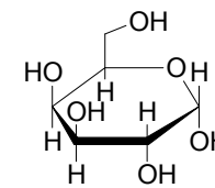
\alpha -D-Galactopyranose
