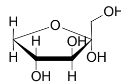
\alpha -D-Xylulofuranose
