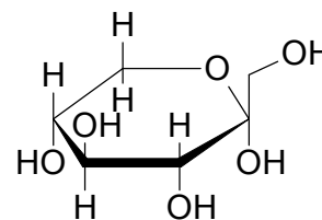
\alpha -D-Sorbopyranose
