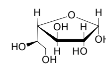
\alpha -D-Galactofuranose
