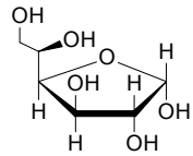
\alpha -D-Glucufuranose
